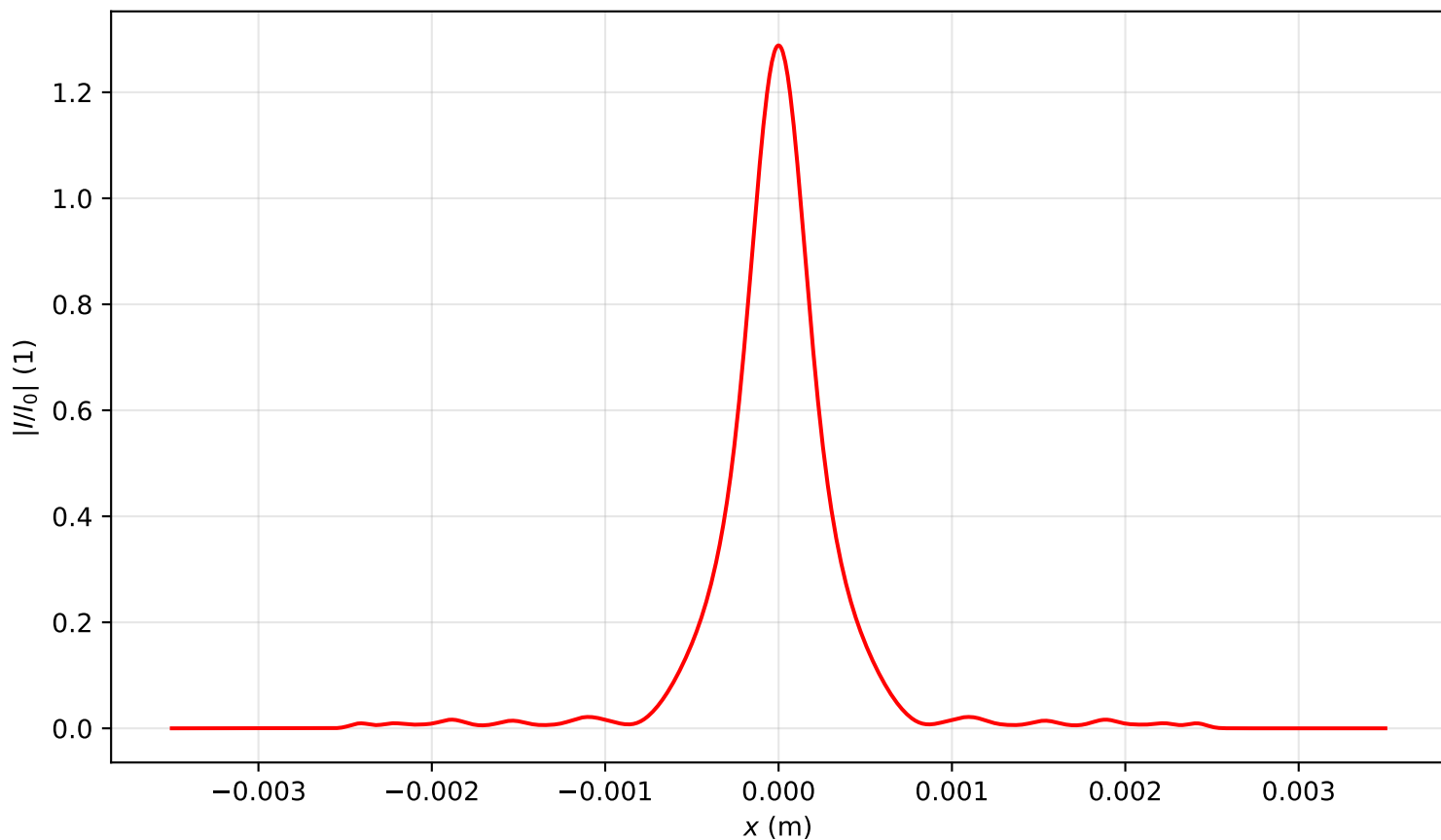
Intensity profile I(x, y = 0, z = 2.866)/I_0 , P_{in}=2.5P_{cr} , artificial time
